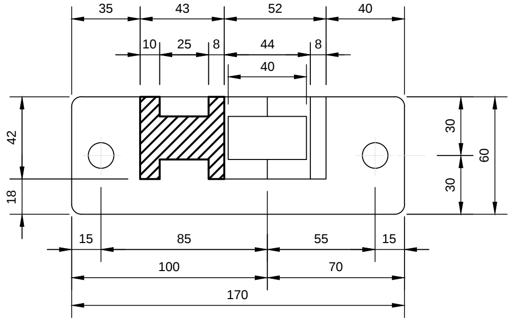
TOP VIEW
